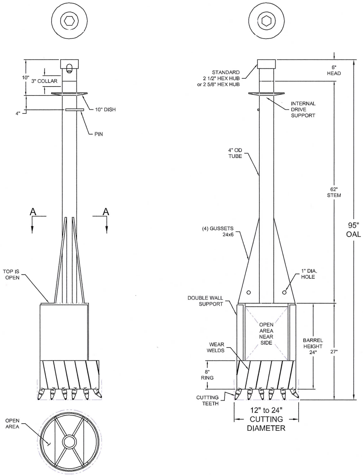
SECTION VIEW "A-A"
